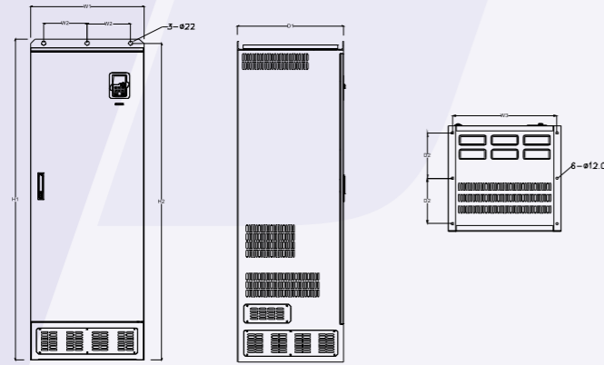
Floor installation of 460V 350G-500G/400P-500P VFDs
