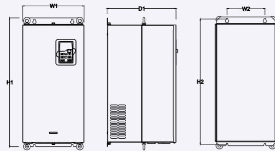
Wall installation of 575V 18.5~110kW VFDs
