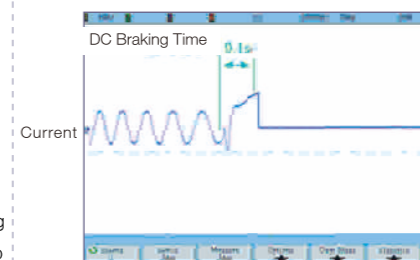
The current waveform in asynchronous motor SVPWM control mode with 100% braking current when the starting frequency is 10Hz and the braking time is 0.1s.
