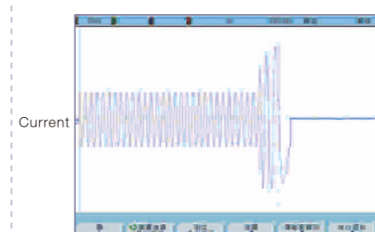
Flux braking current waveform when the running frequency is 50Hz, deceleration time is 0.1s with full load in asynchronous motor SVPWM control mode
